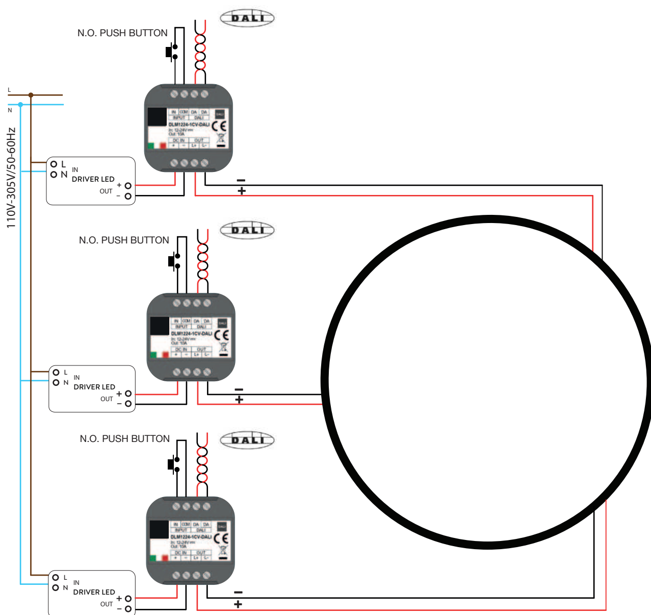
Collegamento in parallelo Parallel connection
