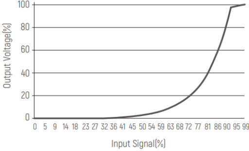
0/1-10V Curve
