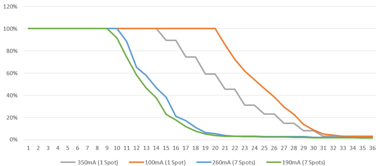
Dimmkurve RLC 350mA
